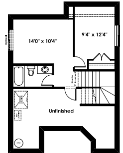
Optional Basement Room Layout for Optional Extended Garage 416 Sq. Ft. (Finished)
