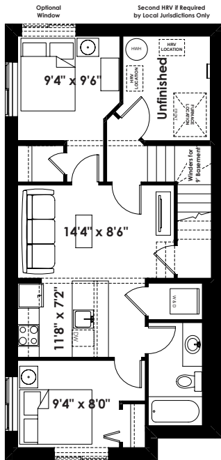
Optional 2 Bedroom Basement Suite Layout 571 Sq. Ft. (Finished Area; Must Add Optional Side Entry; Not Available with Dropped Entries)
