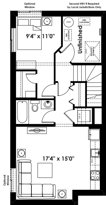
Optional 1 Bedroom Basement Suite Layout 577 Sq. Ft. (Finished Area; Must Add Optional Side Entry; Must Add 9' Foundation Walls; Not Available with Dropped Entries)
